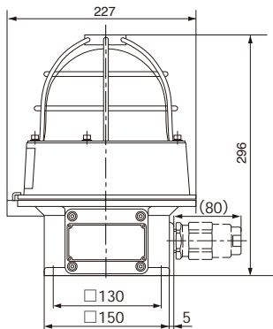
Mounting Dimension
